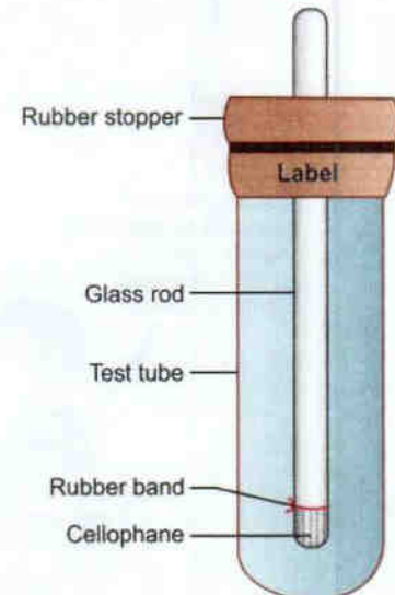
Fig. 4: National Institutes of Health (NIH) swab. A piece of transparent cellophane is attached with rubber band to one end of a glass rod, which is fixed on a rubber stopper and kept in a wide test tube
