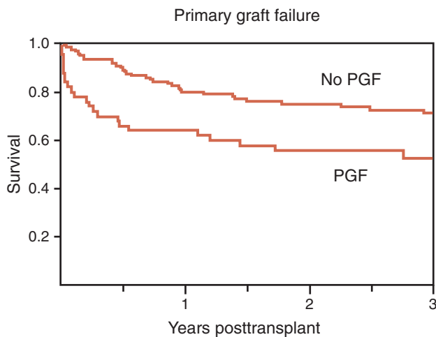
Figure 19-37. The survival rate after lung transplantation at the University of Minnesota as a function of primary graft failure (PGF).
