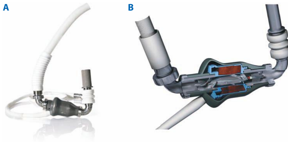
Figure 21-12. The HeartMate II LVAD viewed from the (A) outside and (B) inside. The device is an axial flow, rotary pump that produces no pulsatile action. The pump contains a magnet, and the rotor assembly functions by the electromotive force generated by the motor. The result is that blood is propelled from the inflow cannula to systemic circulation at flows up to 10 L/min. (Images reprinted with the permission of Thoratec Corporation.)
